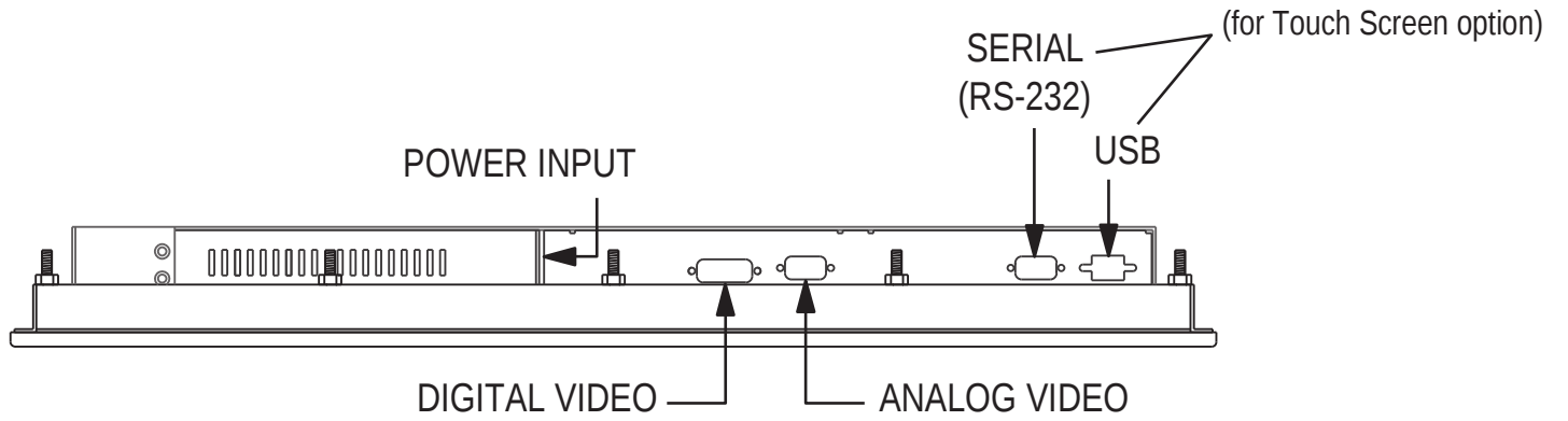
Bottom View
